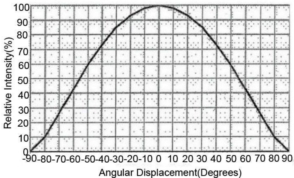
MR16 Beam Pattern
